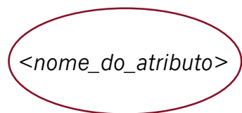
Atributo
